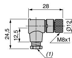
XZ CC8FCM30S
