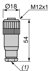
XZ CC12FDM50B
