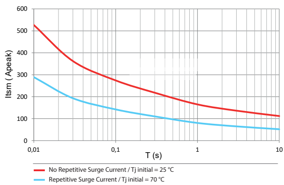
GNR3 - 25 A
