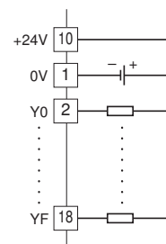
Output Connection Example
