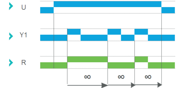
Function TL - Latching (Alternating) – Leading Edge
