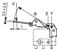
55C large overtravel, flat
