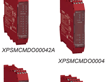
XPSMCMDO0002 XPSMCMDO0004
