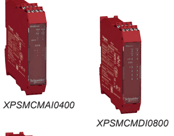
XPSMCMX0802 XPSMCMX0804
