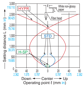
Reflective type
