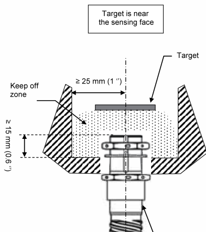
Figure 3 Keep off zone for embeddable switches
