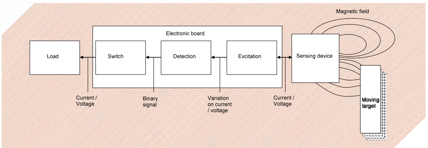
Figure 1 Measurement chain
