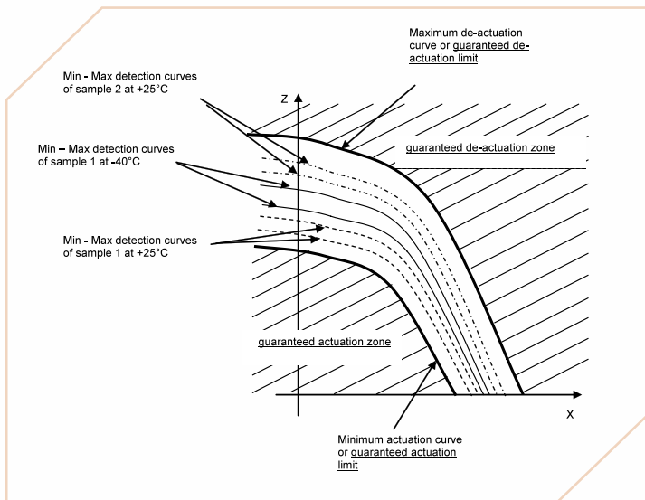
Figure 5 Definition of guaranteed detection curve and zones
