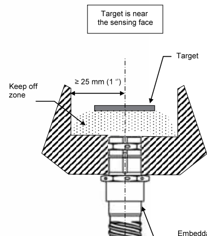
Figure 2 Keep off zone
