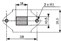
Square lever
