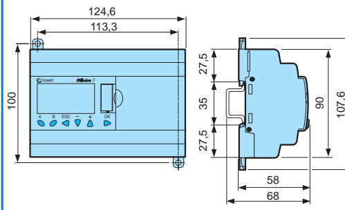
XD26 Smart
