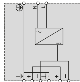
ABL 8REM24050
