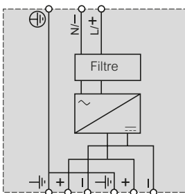
ABL 7RP1205/48030
